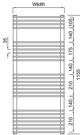
Pearl 1155 High
