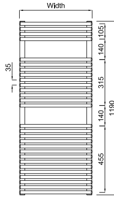
Topaz 1190
