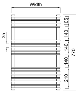
Pearl 770 High
