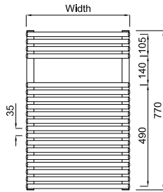
Topaz 770
