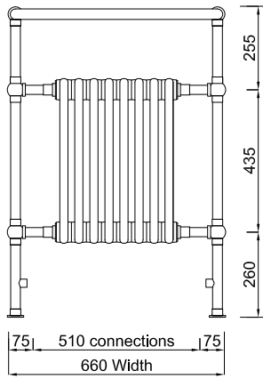
Tuscany Elevation
